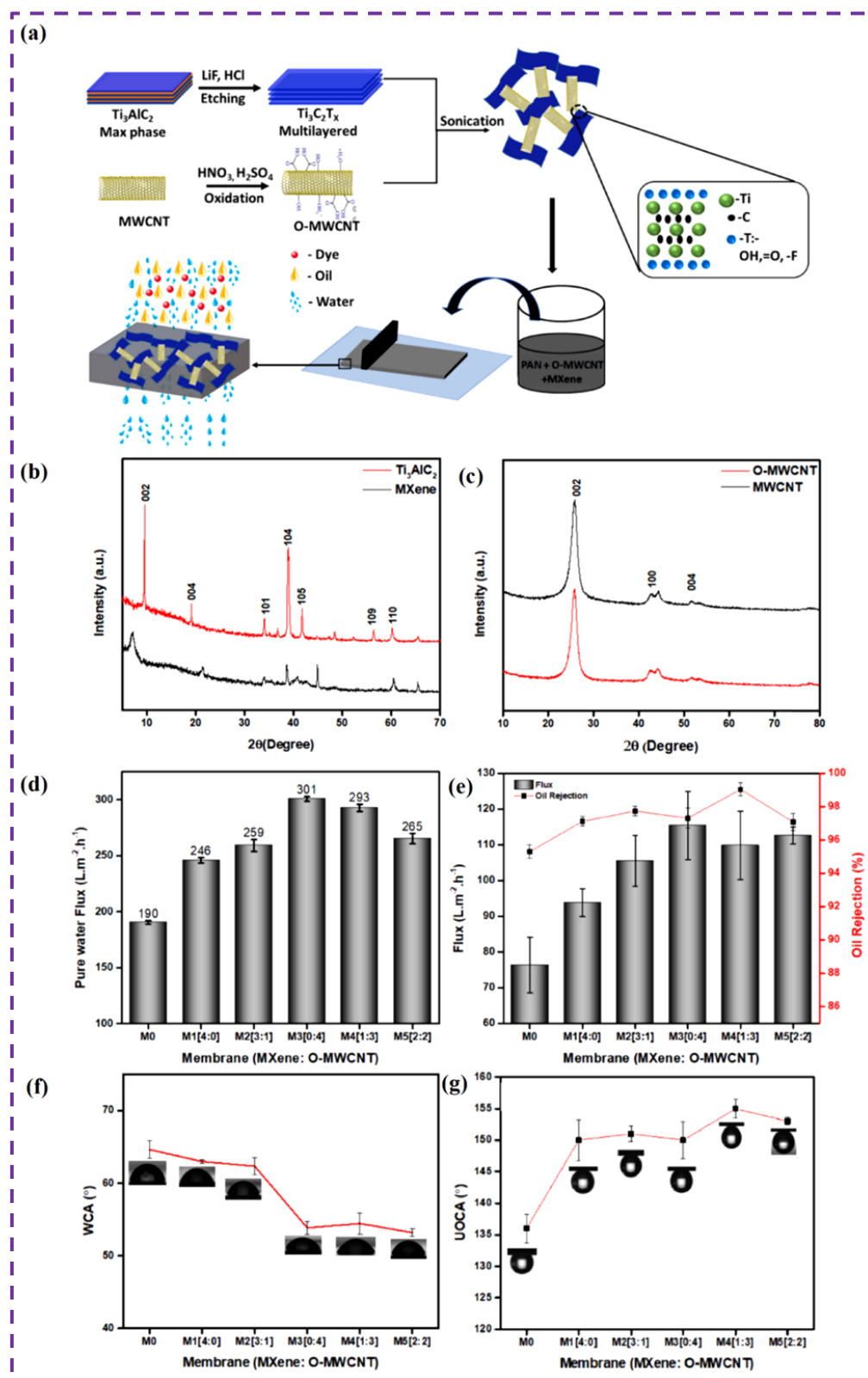
Figure 15. (a) Fabrication of MXene/O-MWCNT@PAN composite membrane for removal of complex oily waste emulsion. (b,c) XRD patterns for (b) \text{Ti}_3\text{AlC}_2 and MXene, and (c) MWCNT and O-MWCNT. (d) Pure water flux for M0-M5. (e) Flux and rejection for oil and water separation. (f) Water contact angle for membrane M0-M5. (g) Underwater oil contact angle for membrane M0-M5. Reprinted with permission [120]. Copyright 2021 Elsevier.
