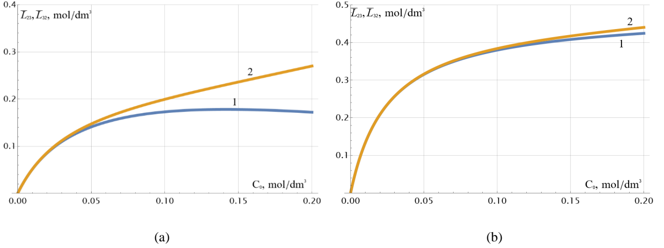
Figure 4. Exact calculated dependences of normalized electrodiffusion coefficients \bar{L}_{23} = L_{23} RT/(FD_+) —curves 1 and \bar{L}_{32} = L_{32} RT/(FD_+) —curves 2 for cast perfluorinated MF-4SK membrane depending on concentration C_0 of an aqueous solution of NaCl (a) and the MF-4SK extrusion membrane (b).
