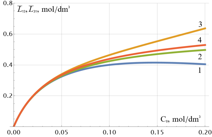
Figure 3. Calculated dependences of the normalized capillary osmotic \bar{L}_{13} = (\mu^\circ/k_D)L_{13} —1,2 and reverse osmotic \bar{L}_{31} = (\mu^\circ/k_D)L_{31} —3,4 coefficients for the cast perfluorinated MF-4SK membrane on the concentration C_0 of an aqueous NaCl solution at \gamma = 0.527 —1,3; \gamma = +\infty —2,4 (ideally selective cation exchange membrane).
