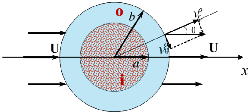
Figure 2. Single cell of the membrane: i—charged porous spherical particle; o—spherical layer of electrolyte solution; U —filtration rate; x —flow direction.
