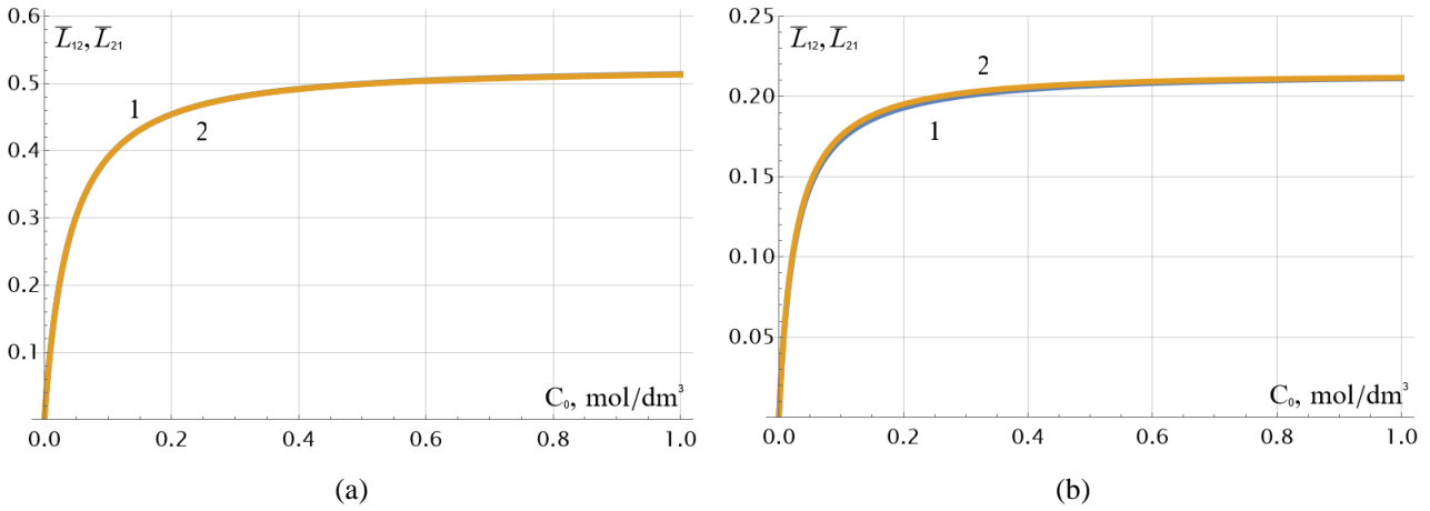
Figure 5. Exact calculated dependences of the dimensionless electroosmotic coefficient \bar{L}_{12} = L_{12} RT/(FD_+) —curves 1 and the coefficient determining the streaming current \bar{L}_{21} = L_{21} RT/(FD_+) —curves 2 for MF-4SK cast perfluorinated membrane depending on concentration C_0 of aqueous NaCl solution (a) and the MF-4SK extrusion membrane (b).
