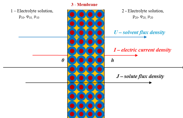
Figure 1. Membrane cell for the study of nonequilibrium processes: 1 and 2—giving and receiving chambers, 3—membrane as an assembly of porous charged particles.
