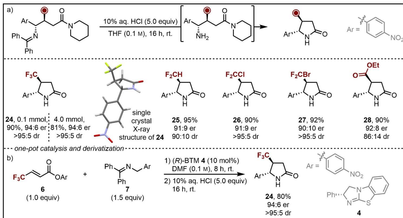
Figure 3. Reaction scope of the Michael addition/hydrolysis/lactamisation cascade. (a) Hydrolysis and cyclisation of the Michael addition product. Reaction carried out at 0.1 mmol scale; all yields are isolated product yields; dr determined by ^1\text{H} and ^{19}\text{F}\{^1\text{H}\} NMR analysis of the crude reaction mixture; er determined by HPLC analysis on a chiral stationary phase; (b) One-pot catalysis and in situ hydrolysis/cyclization.
