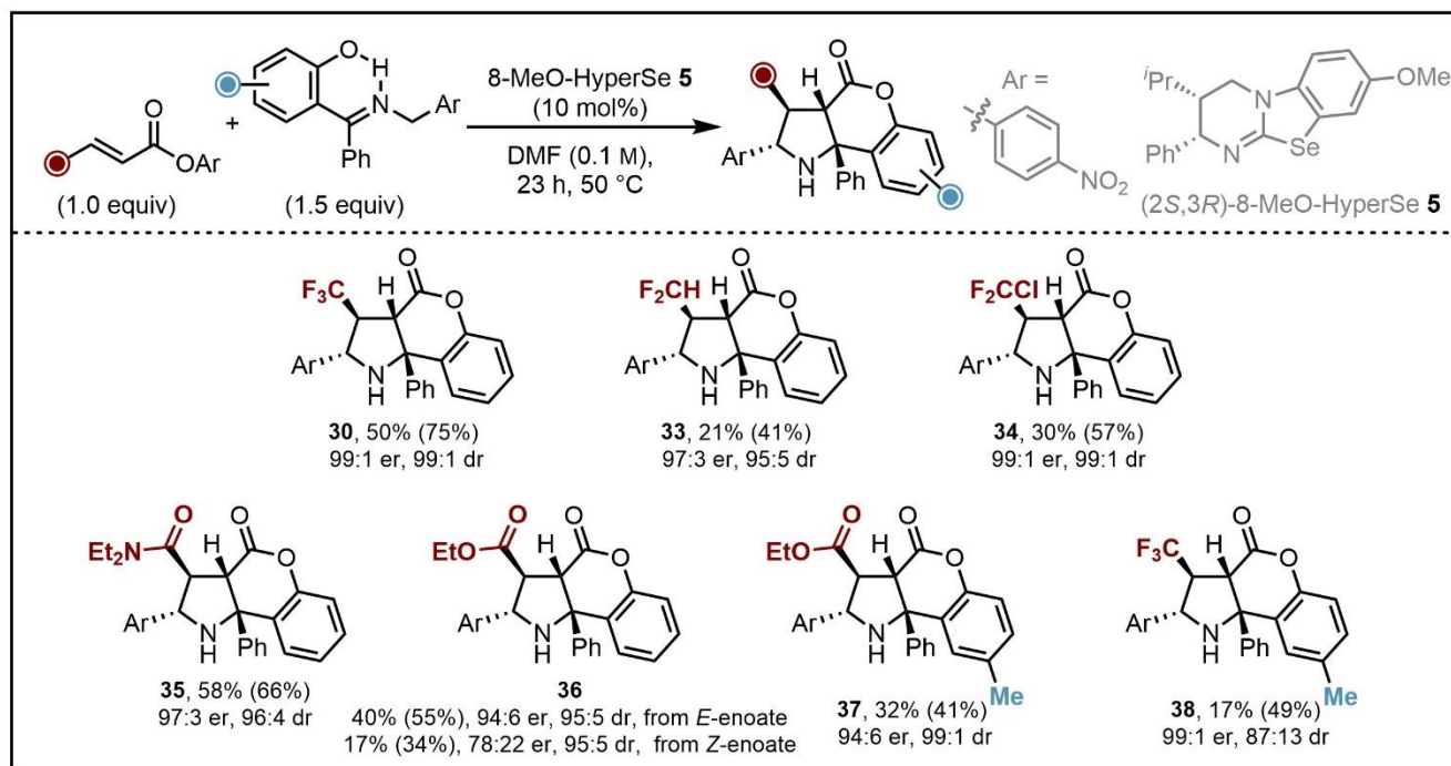
Figure 4. Scope for the Michael addition/Mannich/lactonisation cascade; Reaction carried out at 0.2 mmol scale; isolated yield is given without parentheses; Yields given in parentheses were obtained by 1 H NMR analysis of the crude reaction mixture with 1,3,5-trimethoxybenzene as internal standard, yields not in parentheses are isolated yields; dr determined by 1 H and 19 F{ 1 H} NMR analysis of the crude reaction mixture; er determined by HPLC analysis on a chiral stationary phase.
