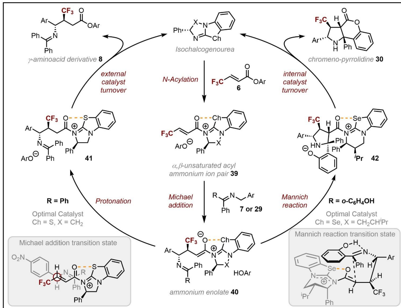
Figure 5. Proposed reaction mechanism.
