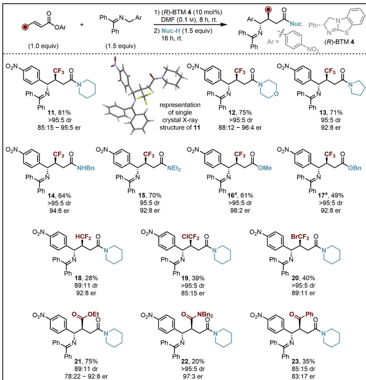
Figure 2. Reaction scope of the Michael addition; Reaction carried out at 0.1 mmol scale; All yields are isolated product yields; dr determined by 1 H and 19 F{ 1 H} NMR analysis of the crude reaction mixture; er determined by HPLC analysis on a chiral stationary phase; a derivatisation in step (ii) used DMAP (20 mol%) as catalyst.
