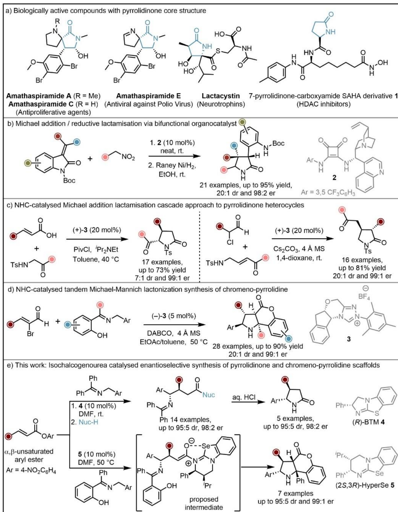
Figure 1. State-of-the-art pyrrolidinone and chromenone synthesis. (a) Importance of pyrrolidinone heterocycles; Enantioselective pyrrolidinone heterocycle synthesis with (b) bifunctional catalyst and (c) NHC catalyst; (d) NHC catalyst in the asymmetric synthesis of chromeno-pyrrolidine heterocycles; (e) This work.
