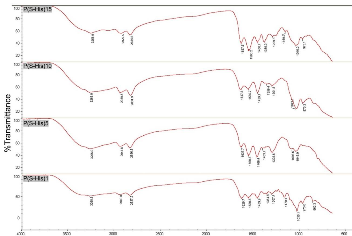
Figure S1. IR spectra of P(S-His) n derivatives.
