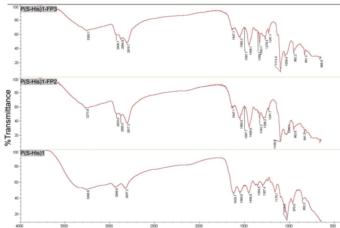
Figure S2. IR spectra of P(S-His)1 and its PEG-FA conjugated derivatives.
