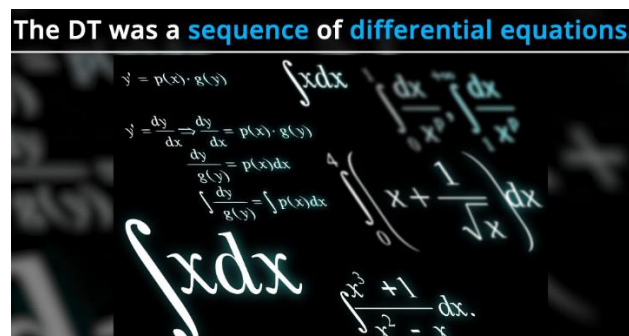
Figure 2. The use of mathematical tools in Digital Twins.
