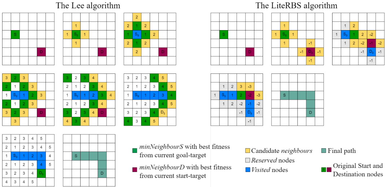
Figure 1. Propagation phases in Lee’s algorithm (left) and the LiteRBS algorithm (right). Lee’s algorithm traverses a large search space of all candidate nodes to identify the shortest path. In contrast, the LiteRBS algorithm selects the most promising node from each direction while reserving the rest to fall back if the current search does not produce a viable path.
