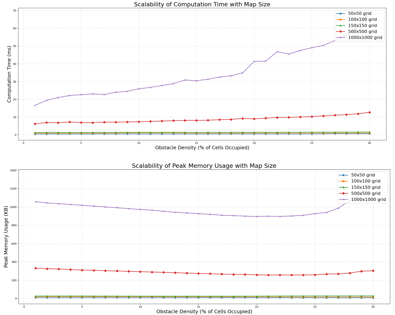
Figure 9. Scalability analysis of the LiteRBS algorithm across varying map sizes ( 50 \times 50 to 1000 \times 1000 ). Plots show computation time (up) and peak memory usage (down), demonstrating stable growth in computational effort as spatial resolution and environmental complexity increase.
