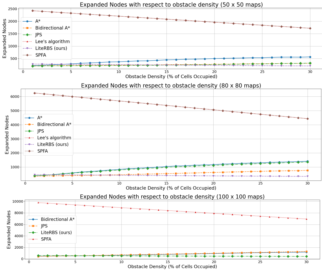
Figure 6. Number of expanded nodes relative to obstacle density in grids of size 50, 80 and 100. The LiteRBS algorithm maintains a flat and density-invariant node expansion, outperforming the baseline, particularly as the environmental noise and spatial complexity scale.
