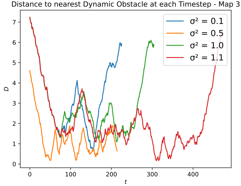
Figure 9. \sigma^2 ablation experiment results.
