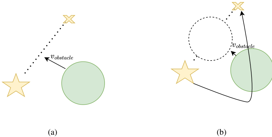
Figure 1. Node connection comparison between proposed RRT algorithm and other RRT algorithms. (a) Node connection in other RRT* algorithms. The predicted position of the obstacle is not considered; (b) Node connection in proposed RRT algorithm. The predicted position of the obstacle is considered.
