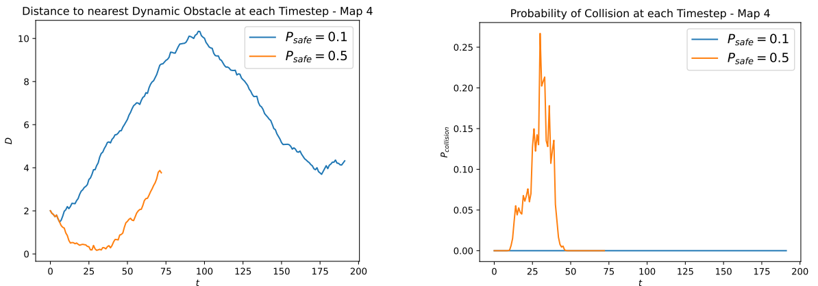
Figure 7. P_{safe} ablation experiment results.
