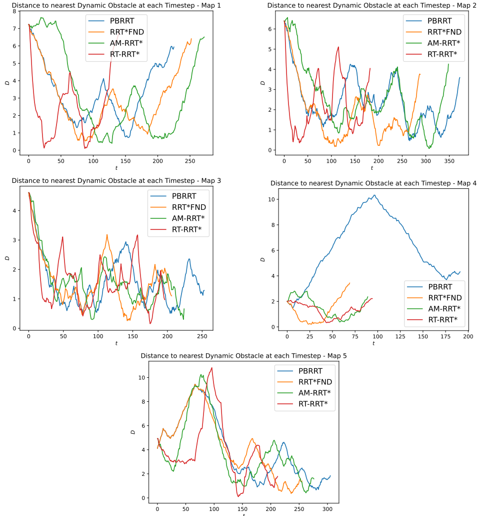
Figure 3. Distances to the nearest dynamic obstacles at each Timestep-Maps 1–5.
