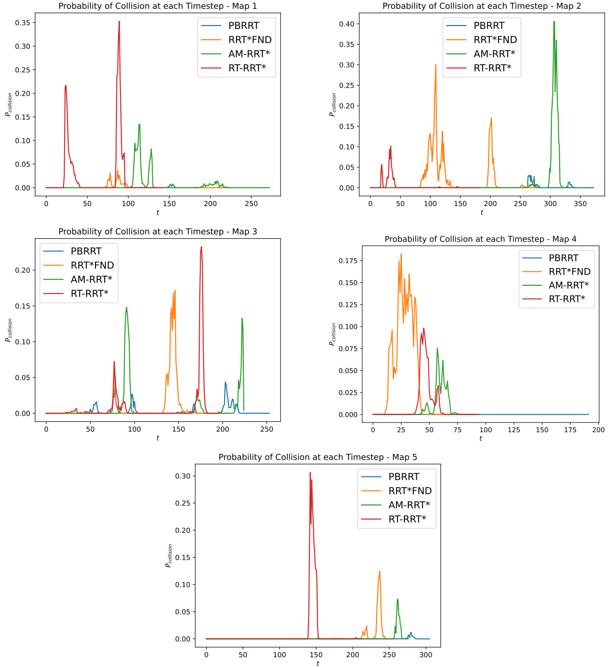
Figure 4. Probability of Collision at each Timestep-Maps 1–5.
