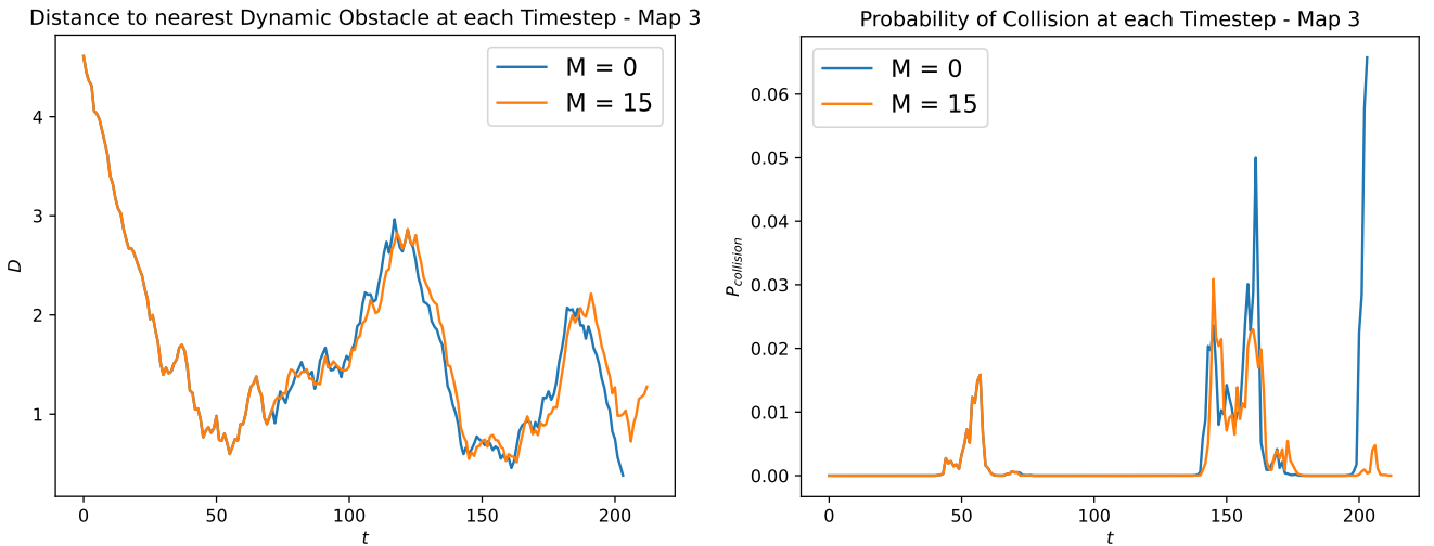
Figure 5. M ablation experiment results.
