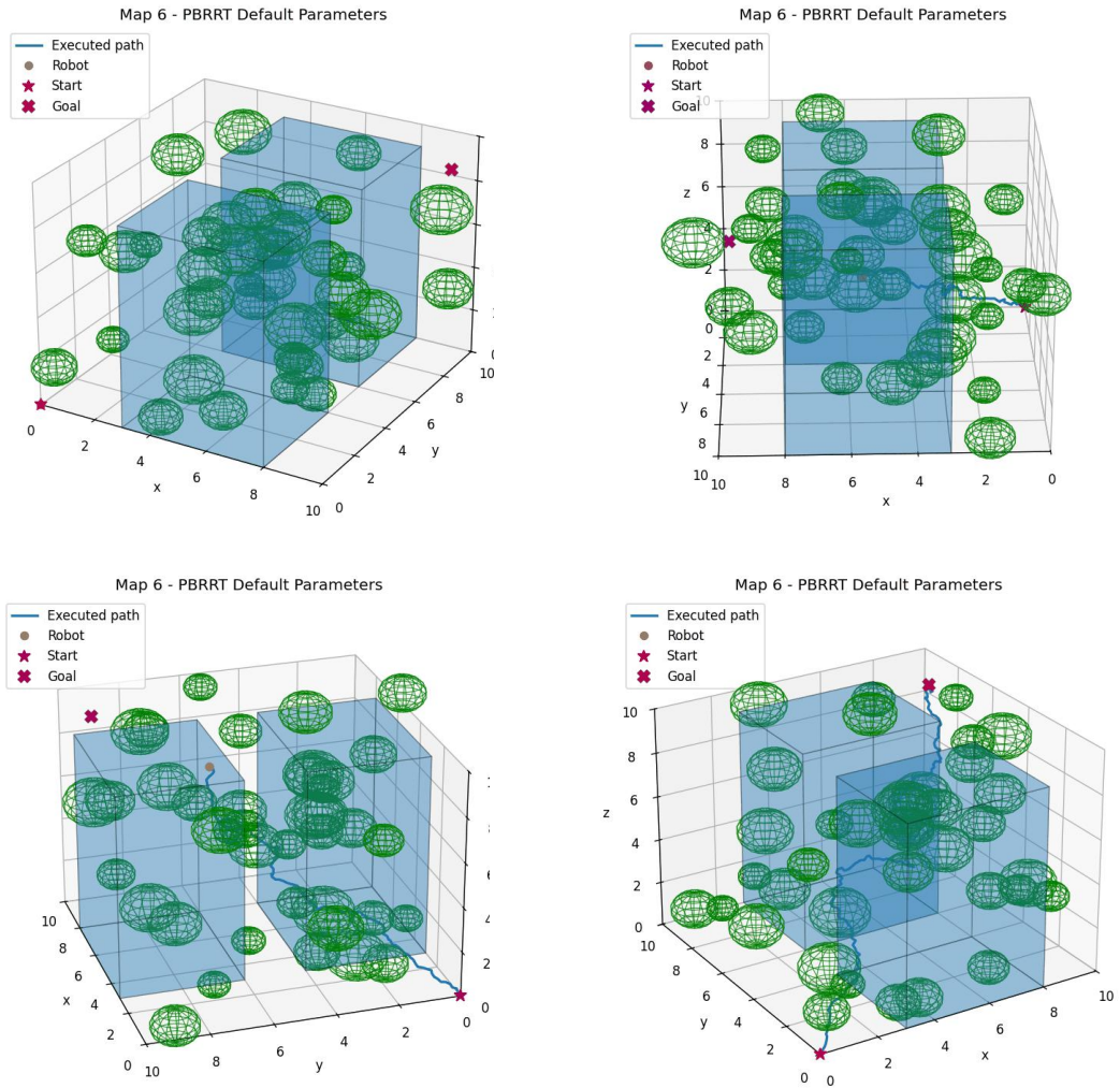
Figure 12. Snapshots of Map 6 executed path with PBRRT default parameters.
