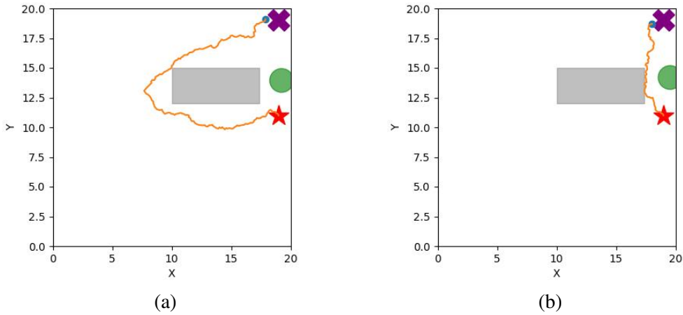
Figure 6. Illustration of executed paths for P_{safe} ablation study. (a) P_{safe} = 0.1 ; (b) P_{safe} = 0.5 .
