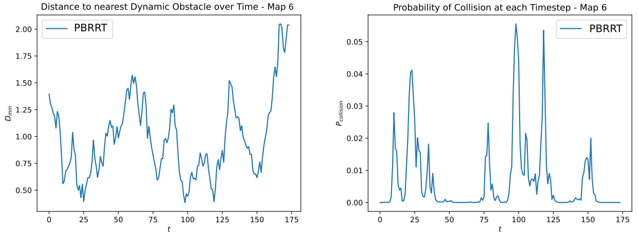
Figure 11. Map 6 DNDO and PoC graphs.
